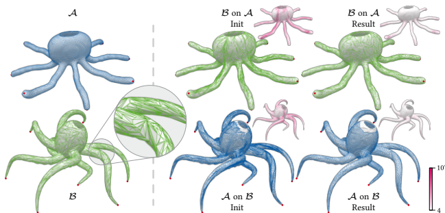
Fig. 10. We map between meshes of different triangulation quality. While \mathcal{A} is uniformly tessellated, we reduced the triangulation quality of \mathcal{B} by a series of edge flips (43% of triangles have an inner angle of less than 10^\circ ). Our method effectively optimizes the initially distorted map and converges within 400 iterations. A logarithmic heat map shows the symmetric Dirichlet energy per polygon before and after the optimization.
