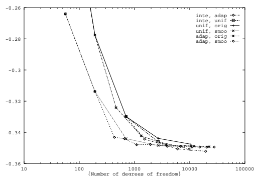
Figure 9: Circular shell with hole, Convergence of midside displacement
