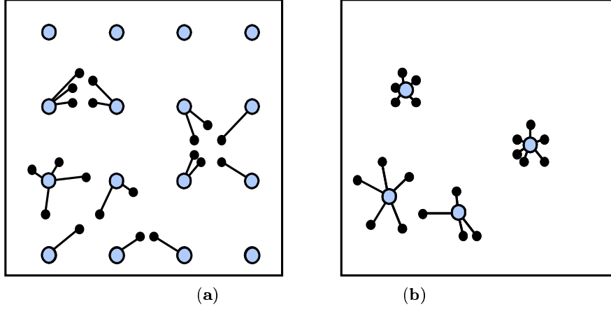
Fig. 11. Quantization of a 20 point dataset (small black circles) in two dimensions. (a) Uniform quantization to 16 levels (large gray circles). Mapping is denoted by lines. Note that only 11 of the 16 quantization levels are used. (b) Non-uniform quantization. Four levels suffice to achieve a quantization error comparable to (a).
